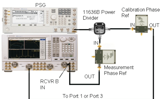
Figure 4-2 Quick-check Configuration for NVNA Test
