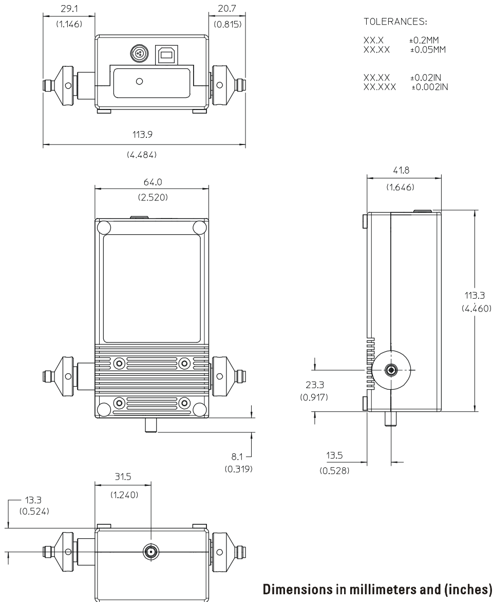
Figure 3-4 Mechanical Dimension of U9391F Comb Generator
