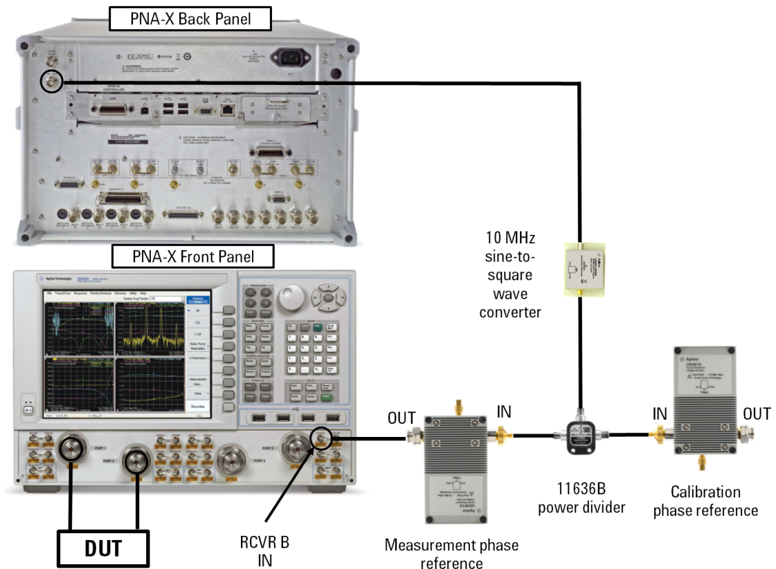
Figure 2-2 U9391F/G and Square Wave Converter Configuration
