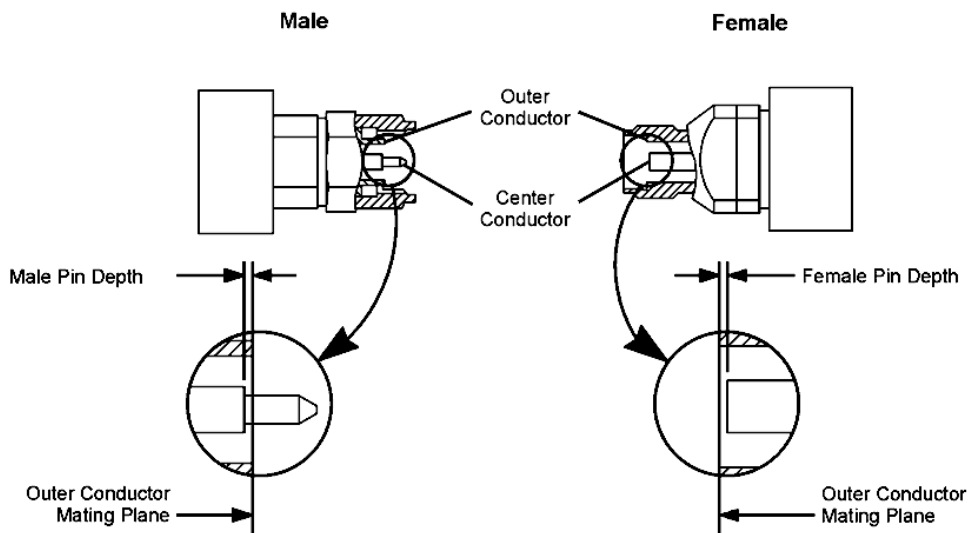
Figure 3-2 Pin Depth for a 1.85mm, 2.4mm, and 3.5mm Connectors
