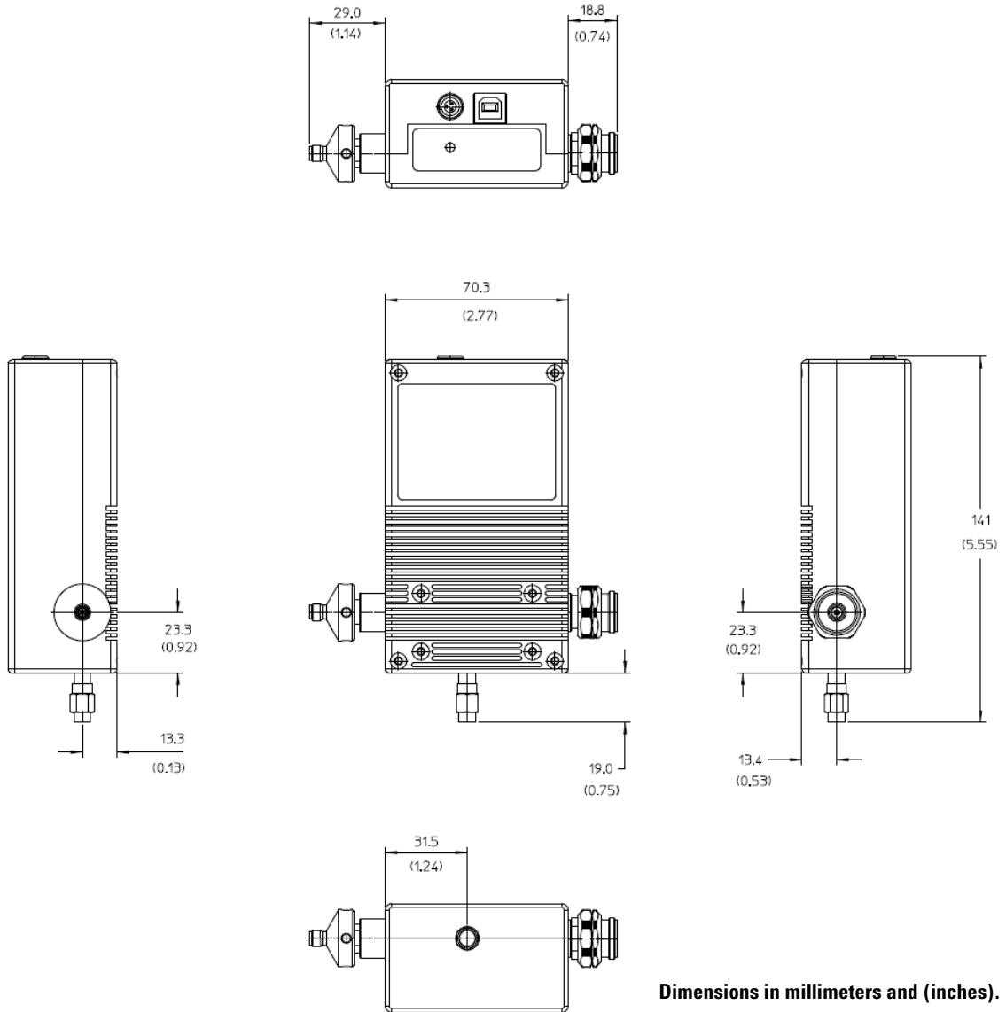
Figure 3-5 Mechanical Dimension of U9391G Comb Generator
