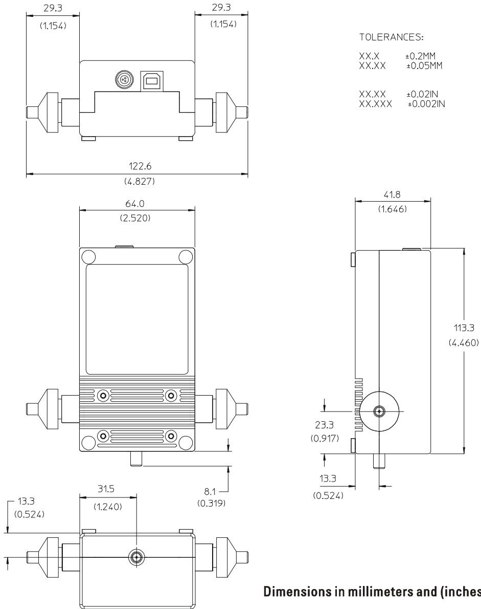
Figure 3-3 Mechanical Dimension of U9391C Comb Generator
