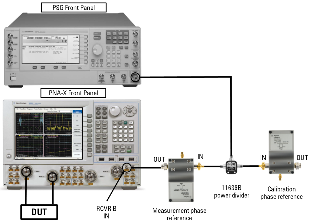
Figure 2-1 U9391C/F/G and PNA-X Configuration
